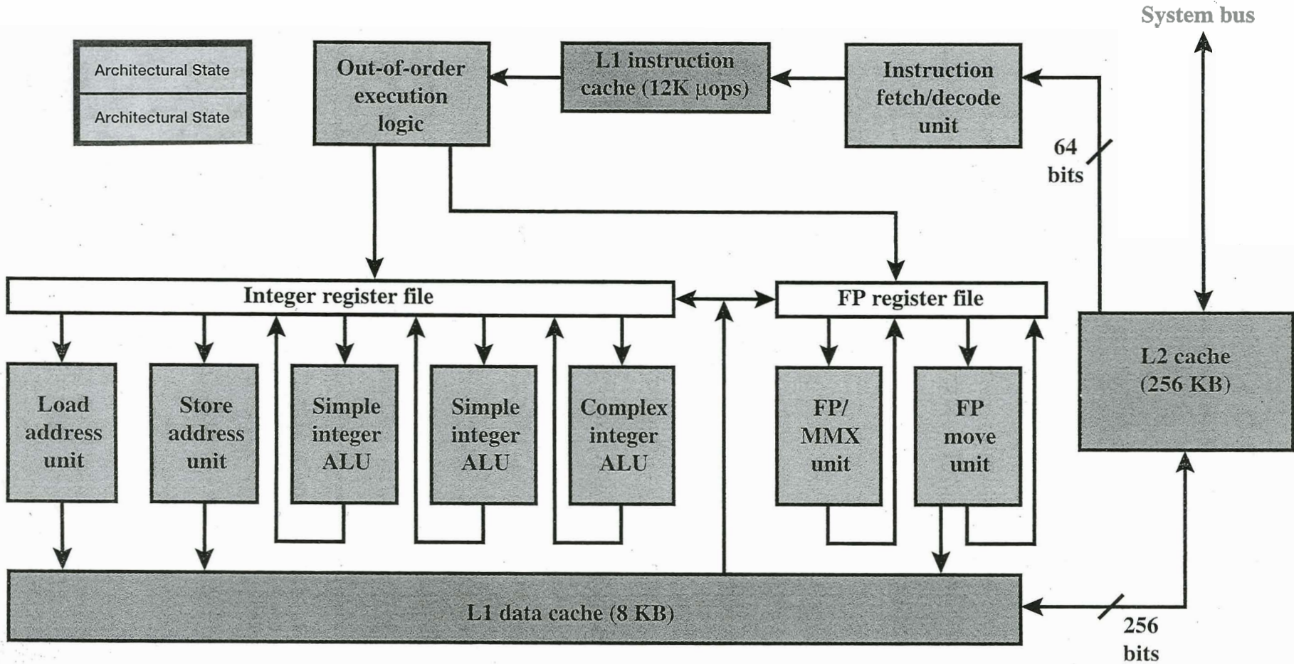
Figure 4.13 Pentium 4 Block Diagram
