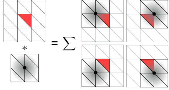
Figure 3: We model convolution as a summation of BT solids. In order to convolve one tetrahedron of a BT Volume, pictured above in red, with a BT Volume filter with the same \kappa function, we need to sum together the contributions of overlapping BT in all possible translations of the filter, each scaled by the sample value at that filter position.
