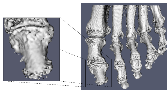
Figure 6: Comparison image using the Marching Cubes algorithm at 128^3 (as implemented by ParaView), showing the rough and noisy nature of Marching Cubes renderings. Inset shows significant linear interpolation artifacts (visible as linear features in the shading and geometry).
