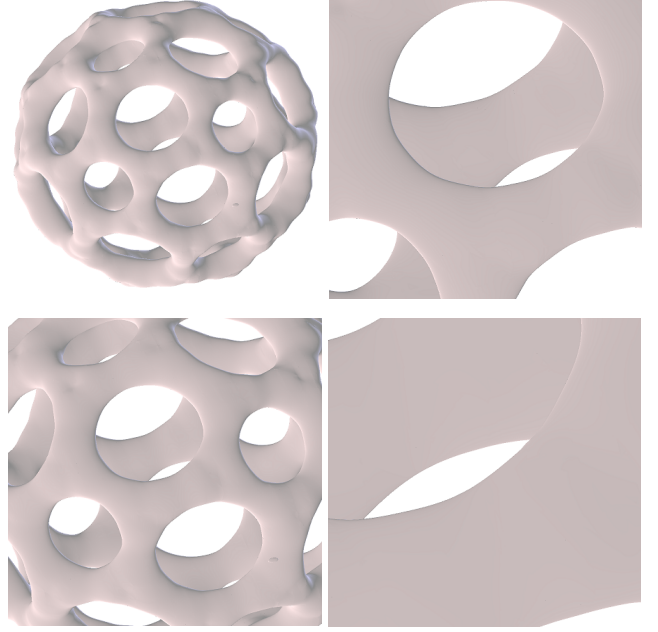
Figure 4: Several shots in a zoom animation of a 32^3 volume reconstruction show the resolution independence of the BT Volume format.
