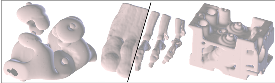
Figure 1: Several renderings of BT Volume data. Left: Real-time isosurface rendering of a molecular simulation. Center: Composition of two real-time isosurface renderings of a foot data set. Our system renders any isosurface level and supports changing the isosurface level in real time. Right: Higher detail rendering of engine block generated offline.
