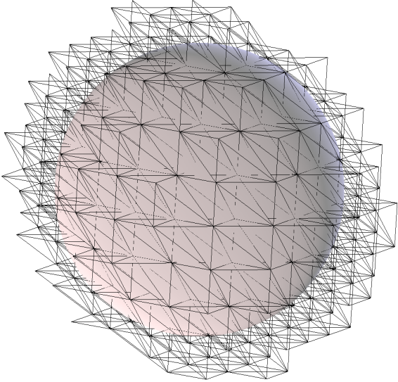
Figure 2: An isosurface rendering of a BT Volume approximating a Gaussian reconstruction filter where lines denote the boundaries between adjacent tetrahedra. Note that tetrahedra which would not contribute to this particular isosurface are culled before rendering. We generate filters which are C^0 continuous and enforce zero values on the boundary.
