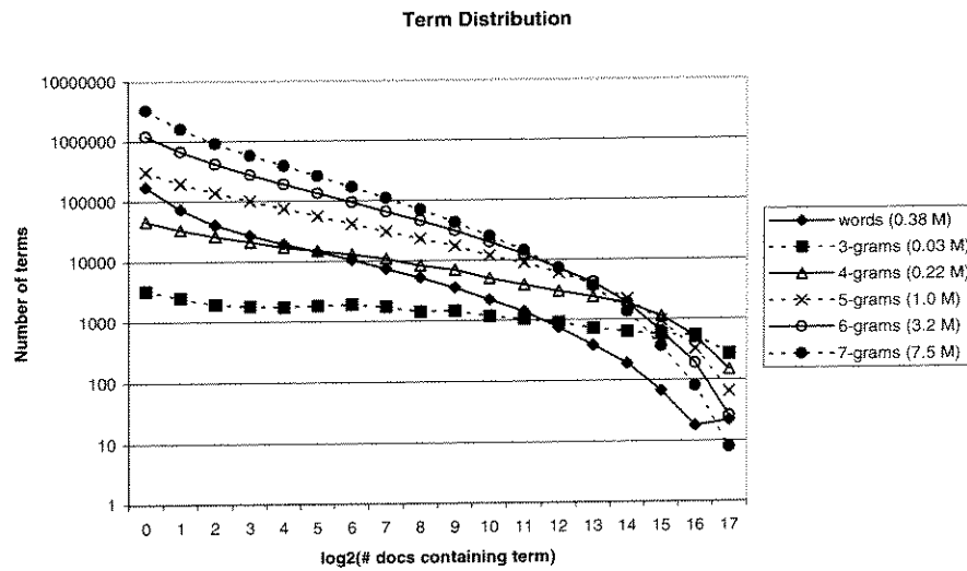
Figure 6. Term distributions in Spanish for multiple indexing units.
